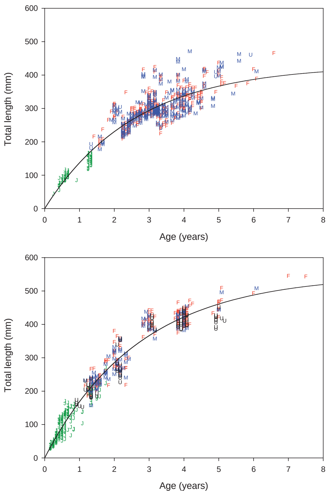
Figure 2.3d. Von Bertalanffy growth curves and age-length data for King George whiting for the south (top) and west (bottom) regions of Western Australia. (F – females, M – males, J – juveniles, U – unknown)
