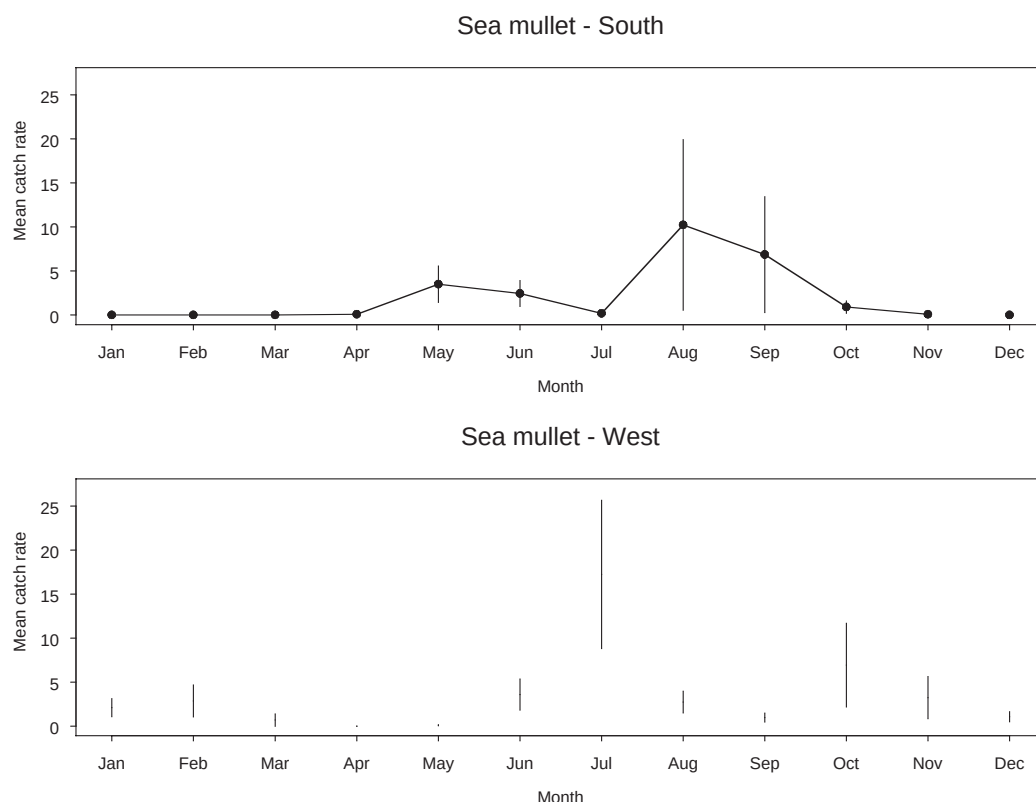
Figure 3.4f. Mean monthly (+ 1 std deviation) 0 + catch rate for sea mullet from the south and west regions of WA between June 1999 and June 2002.
