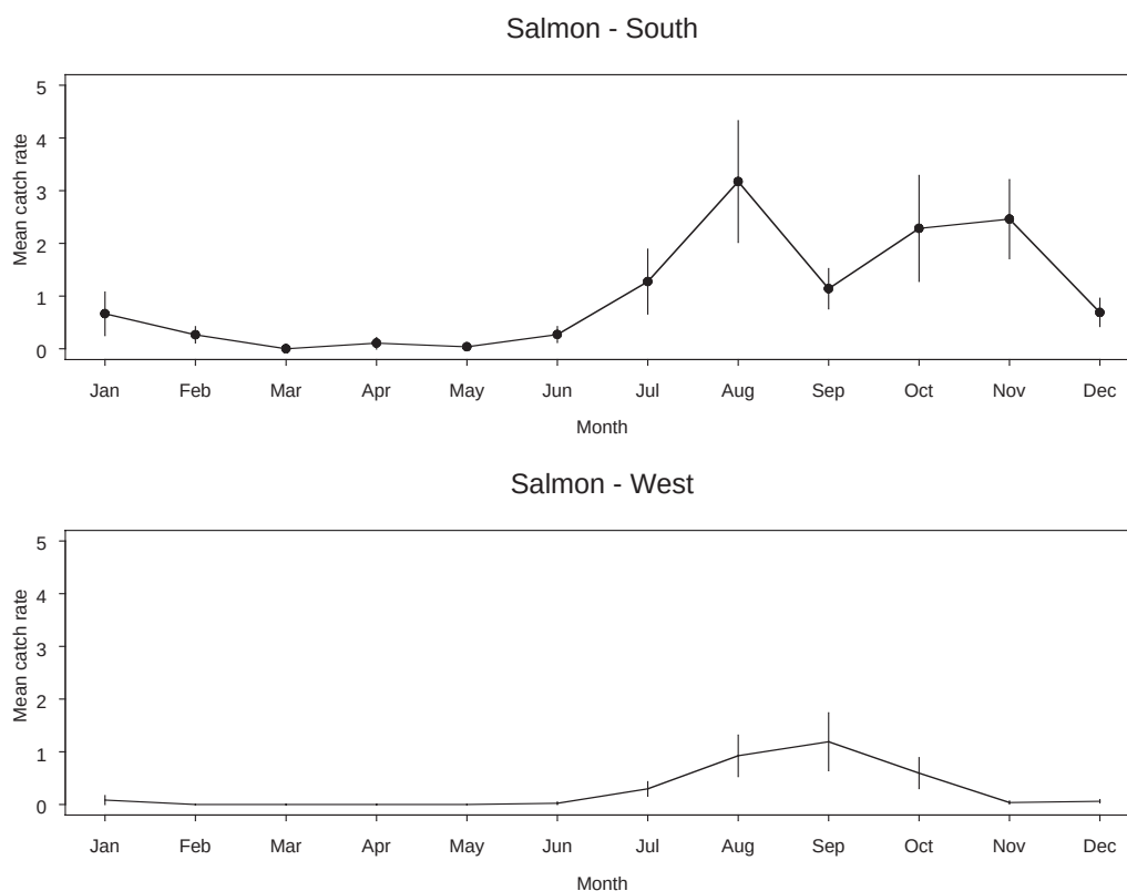
Figure 3.4b. Mean monthly (+ 1 std deviation) 0 + catch rate for Western Australian salmon from the south and west regions of WA between June 1999 and June 2002.
