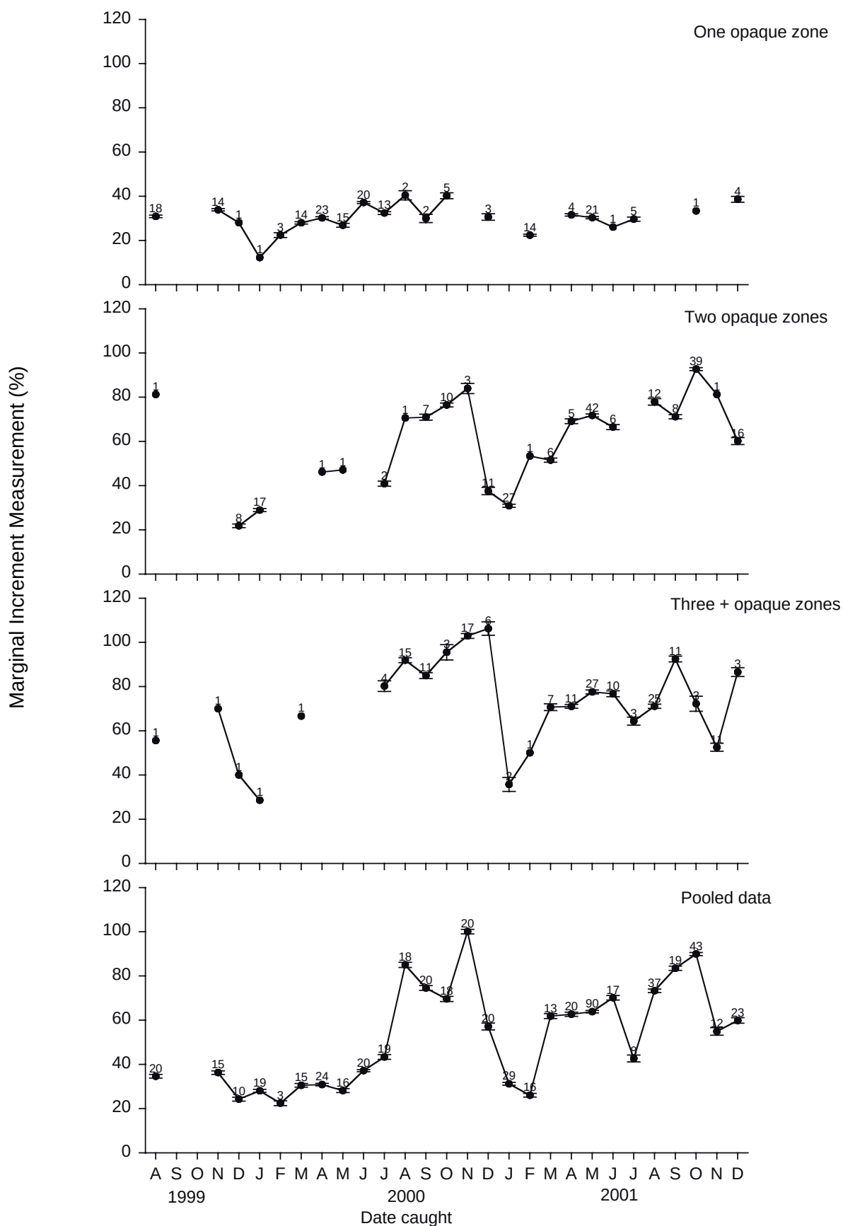
Figure 2.2d Mean monthly marginal increment measurement (%) \pm 1 se for otoliths of sea mullet caught in the south region between August 1999 and December 2001.
