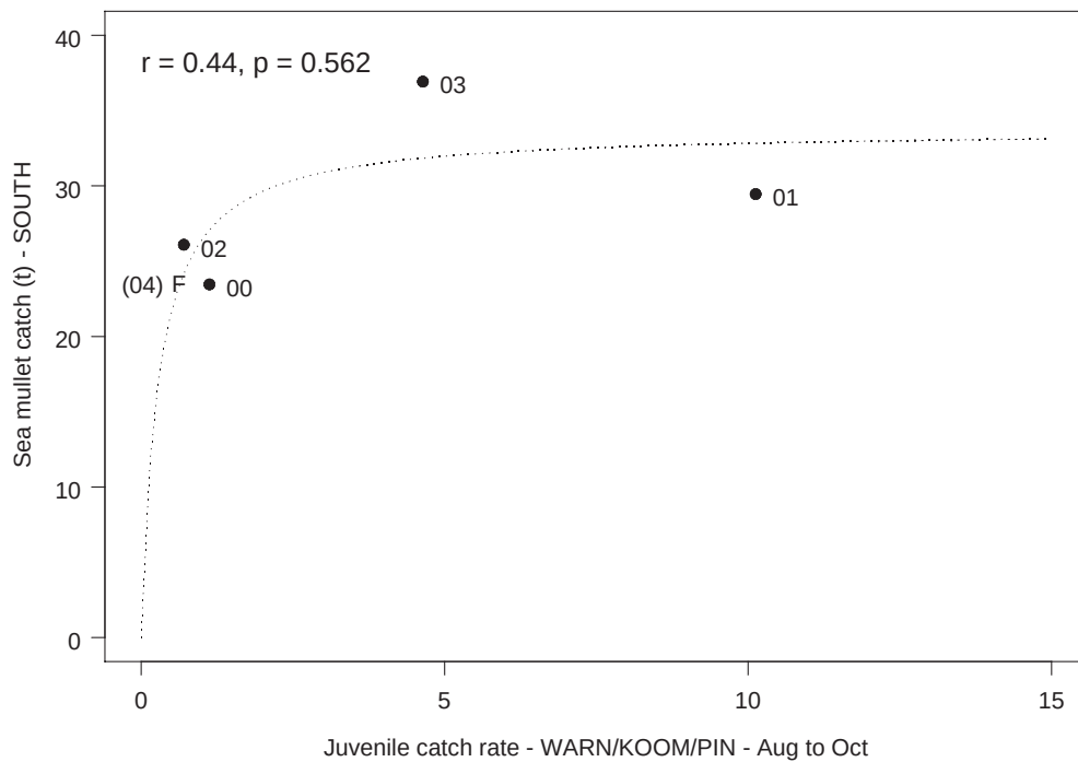
Figure 5.2h. Restricted (3 month maximum) catch rate of sea mullet from combined west coast sites, Warnbro Sound, Pinnaroo Point and Koombana Bay versus the total commercial catch from the south coast applying a 3-4 year time lag. F(04) is the forecast catch for 2004.
