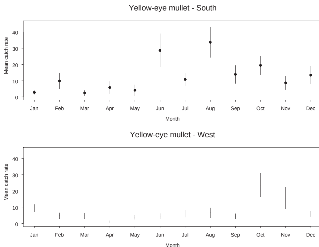
Figure 3.4g. Mean monthly (+ 1 std deviation) 0 + catch rate for yellow-eye mullet from the south and west regions of WA between June 1999 and June 2002.
