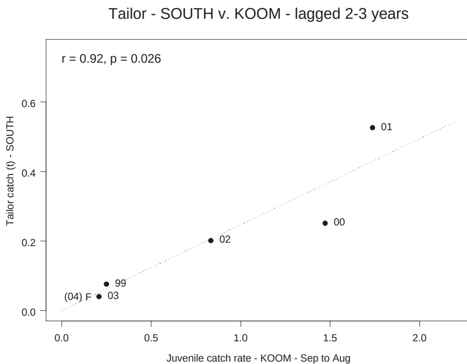
Figure 5.1e. Annual mean recruit catch rate of tailor from west coast site Koombana Bay versus the total commercial catch of tailor from the south region applying a 2-3 year time lag. F(04) is the forecast catch for 2004.
