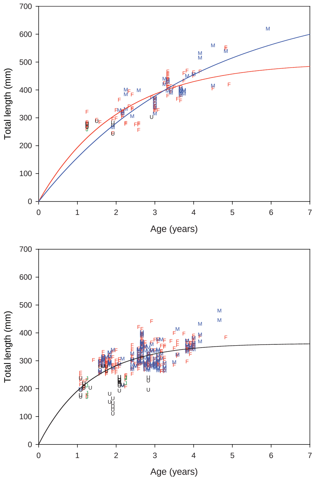
Figure 2.3c. Von Bertalanffy growth curves and age-length data for tailor for the south (top) and west (bottom) regions of Western Australia. (F – females, M – males, J – juveniles, U – unknown)
