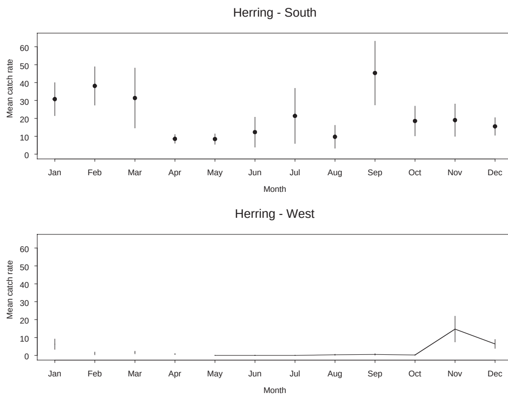
Figure 3.4a. Mean monthly (+ 1 std deviation) 0 + catch rate for Australian herring from the south and west regions of WA between June 1999 and June 2002.
