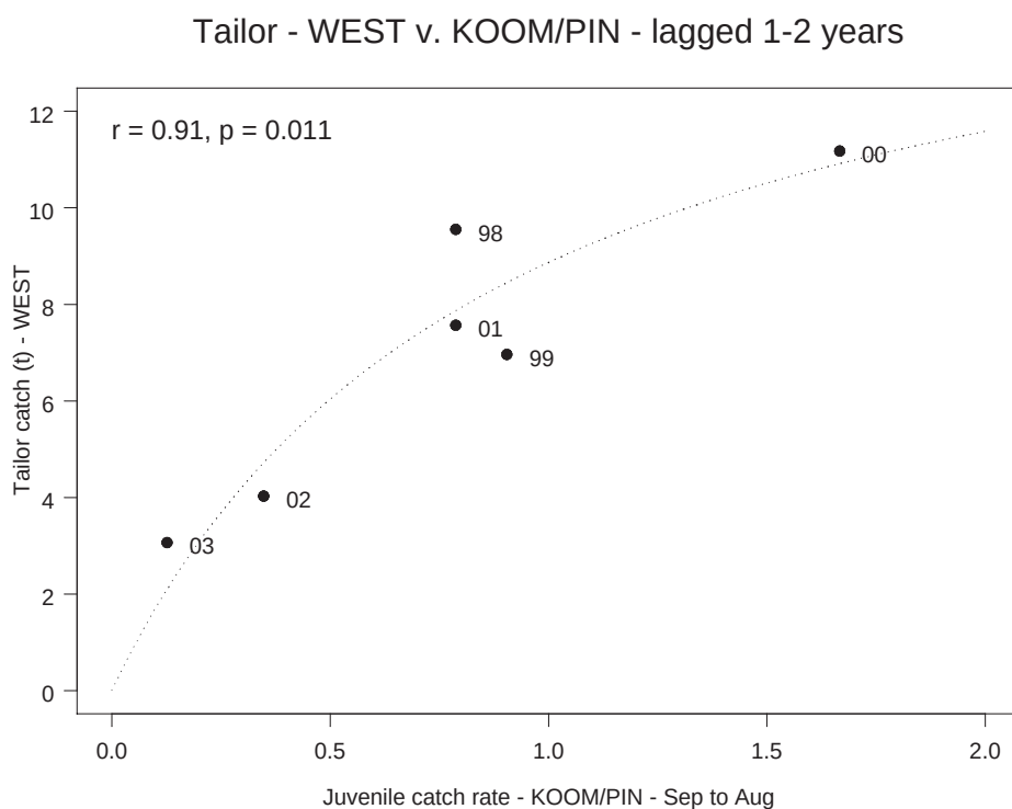
Figure 5.1f. Annual mean recruit catch rate of tailor from west coast sites Koombana Bay and Pinnaroo Point versus the total commercial catch of tailor from the west region applying a 1-2 year time lag.
