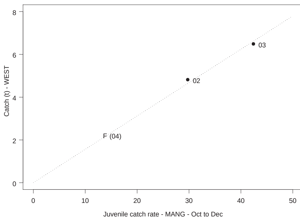
Figure 5.2e. Restricted (3 month maximum) catch rate of King George whiting from west coast site Mangles Bay versus the total commercial catch from the west coast applying a 2-3 year time lag. F(04) is the forecast catch for 2004.
