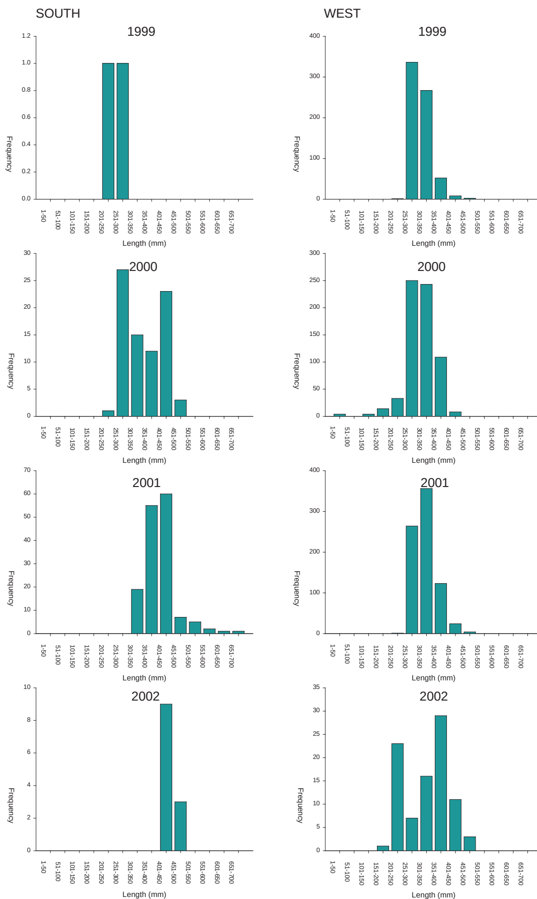
Figure 4.1i. Length frequency (50 mm intervals) of commercial catch of tailor sampled for the west and south regions of WA for 1999 to 2002.
