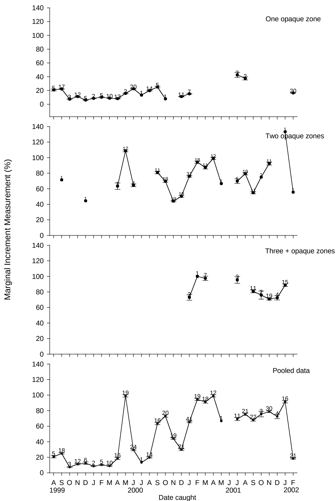
Figure 2.2b. Mean monthly marginal increment measurement (%) \pm 1 se for otoliths of tailor caught in both regions between August 1999 and February 2002.
