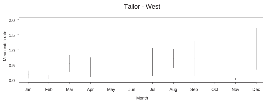
Figure 3.4c. Mean monthly (+ 1 std deviation) 0 + catch rate for tailor from the south and west regions of WA between June 1999 and June 2002.
